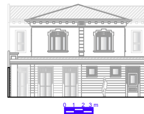
Elevation 03
